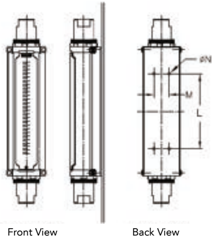
Front of Panel (Wall) Mounting (4 Mounting Holes)
