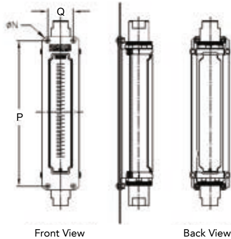
Back of Panel (Flush) Mounting (Rectangular Panel Cut-Out + 4 Mtg. Holes)
