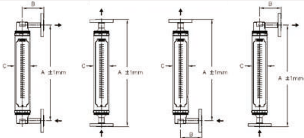
Front View Flanged Connection
