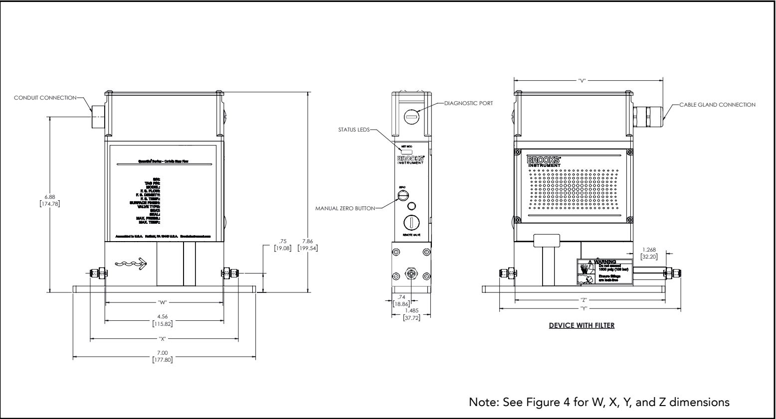
Figure 2 Dimensional Drawing QMC IP6x / Class 1 Division 2 Zone 2
