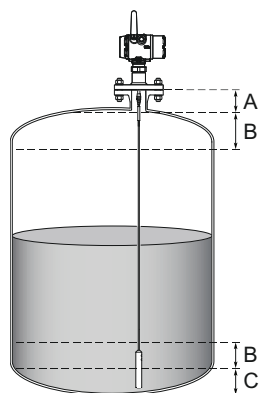
Figure 5: Blind Zones
