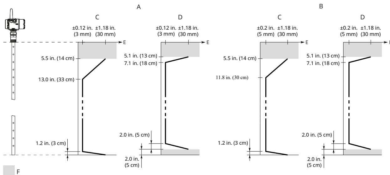
Figure 8: Accuracy over Measuring Range for Coaxial Probe
