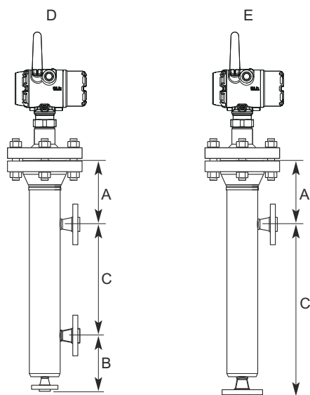
Figure 16: Side-to-Side and Side-to-Bottom Chambers
