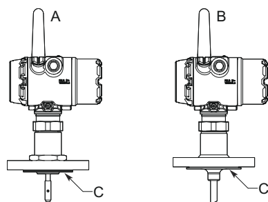
Figure 11: Protective Plate
