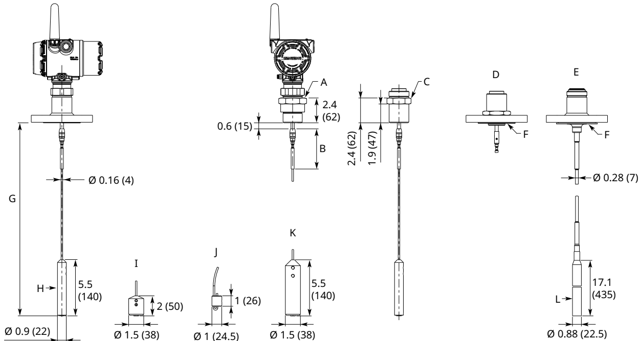
Figure 22: Flexible Single Lead Probe
