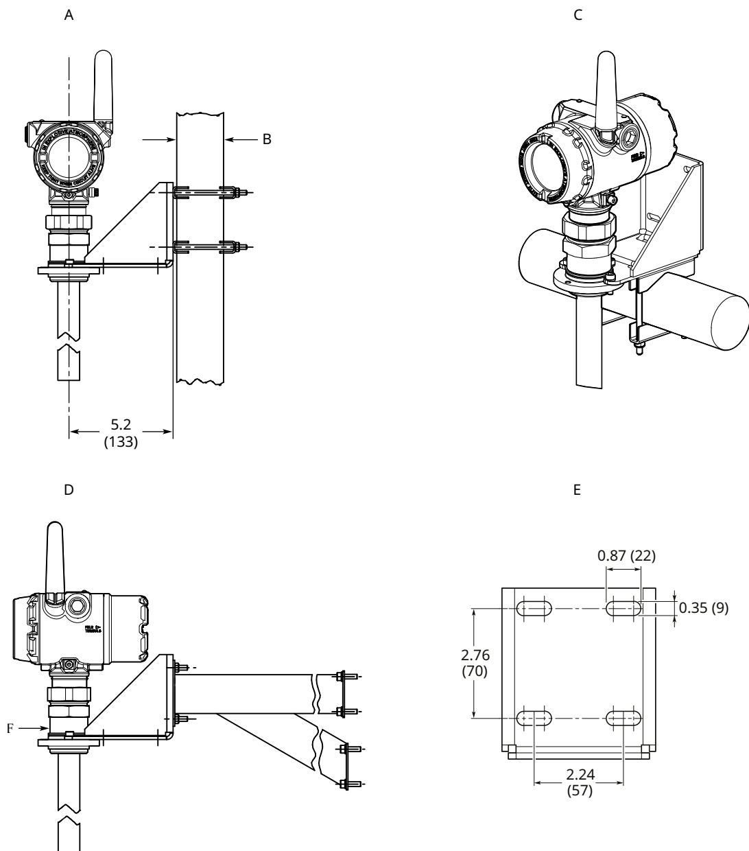
Figure 27: Mounting Bracket (Option Code BR)
