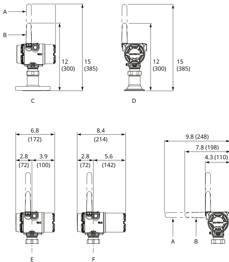
Figure 26: Housing and Antenna
