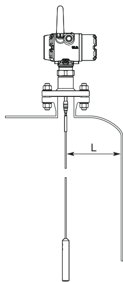
Figure 14: Free Space Requirement
