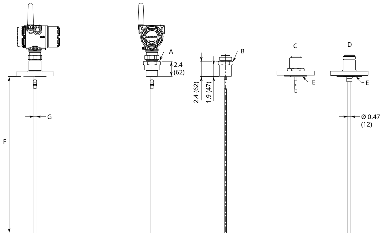
Figure 23: Rigid Single Lead Probe
