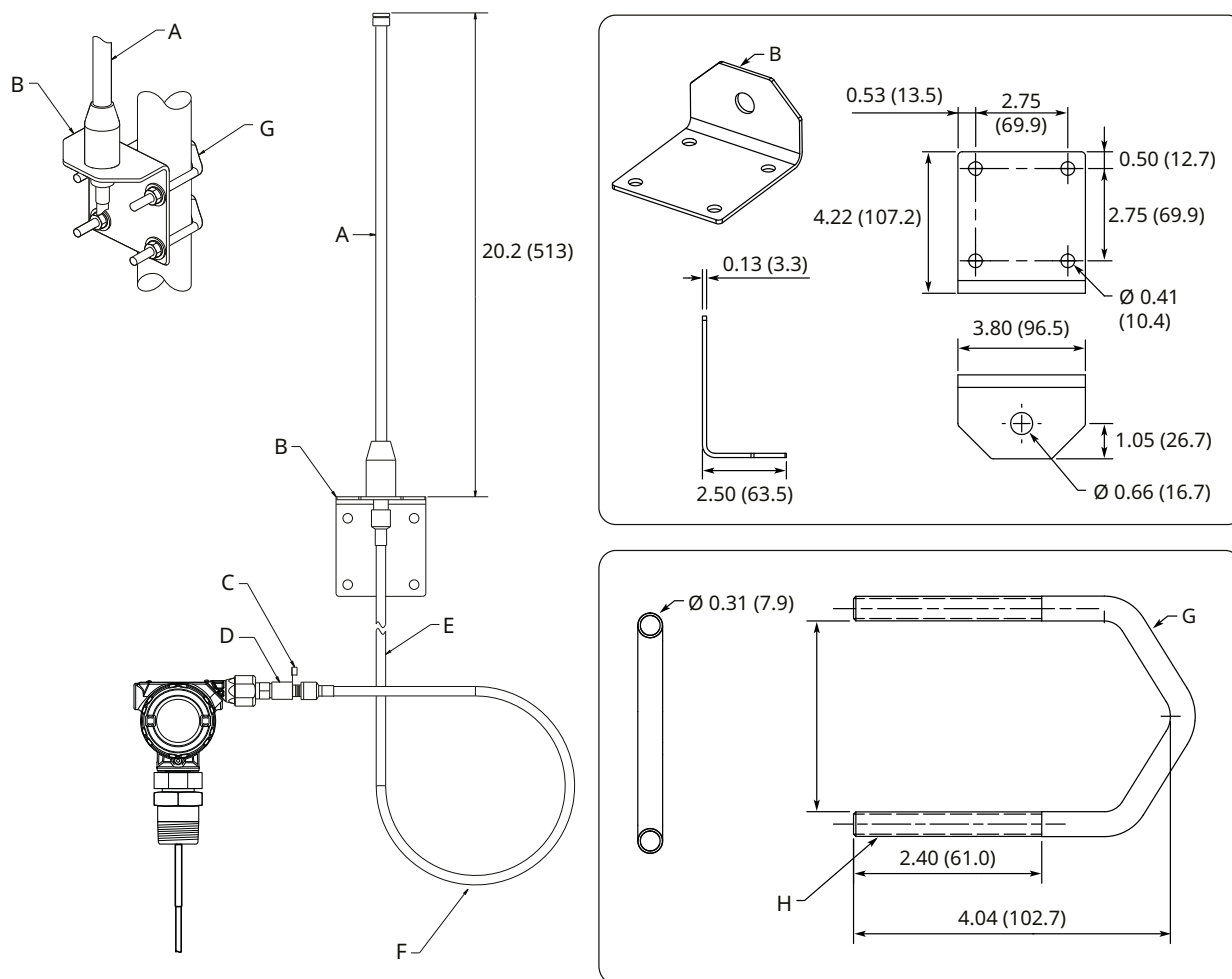
Figure 28: High Gain, Remote Antenna (Option Code WN1 and WN2)
