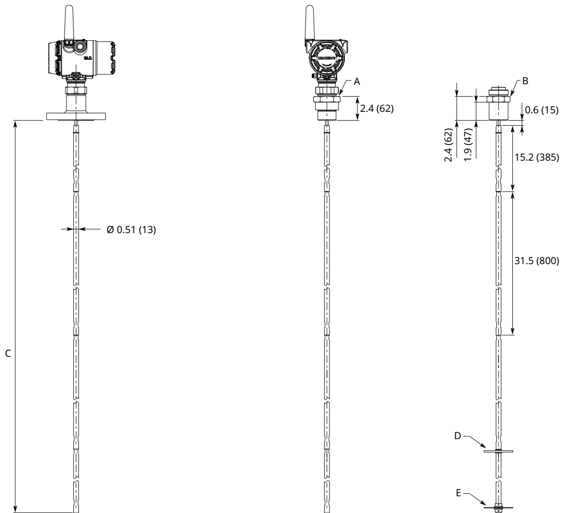
Figure 24: Segmented Rigid Single Lead Probe
