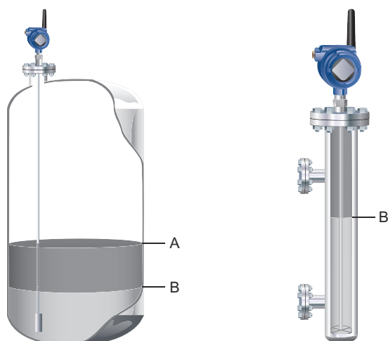
Figure 12: Interface Level Measurement
