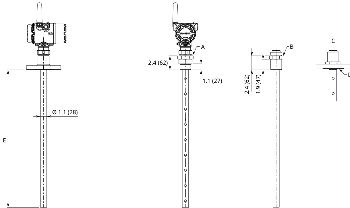
Figure 25: Coaxial Probe
