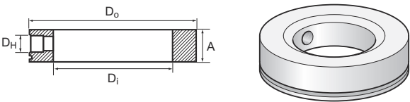
Figure 31: Flushing Connection Rings
