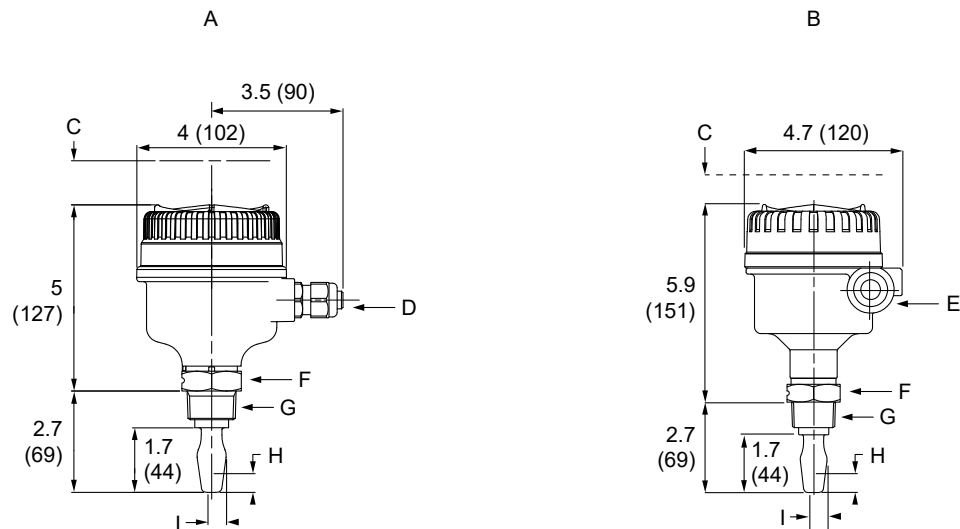
Figure 12: ¾- and 1-in. Threaded Mounting (Standard Length)
