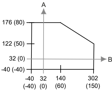
Figure 11: Operating Temperature
