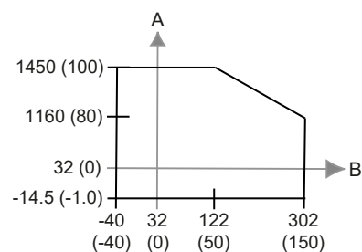
Figure 10: Process Pressure
