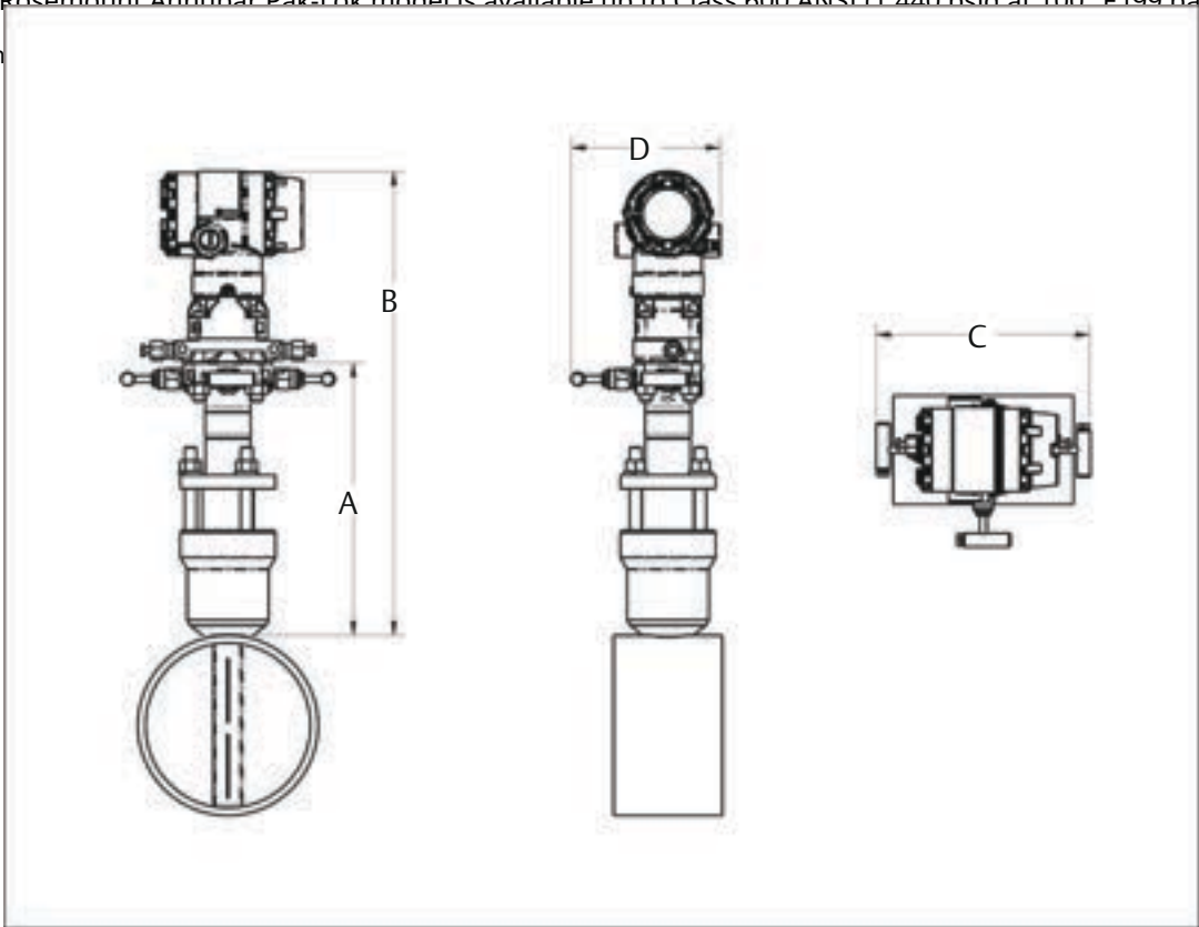
Figure 18: Rosemount 2051CFA Annubar Pak-Lok Flow Meter
