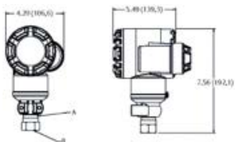
Figure 15: Rosemount 2051 Wireless Housing with In-line Platform
