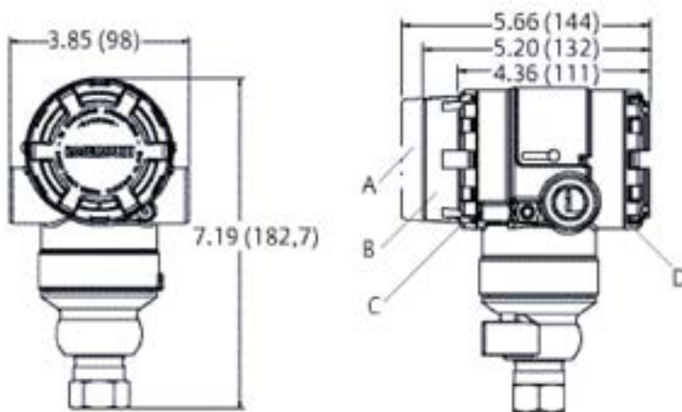
Figure 9: Rosemount 2051T
