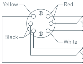
3 Wire Duplex Resistance Thermometer
