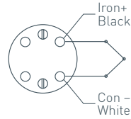
Type J Single Thermocouple
