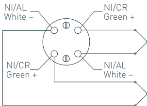
Type K Duplex Thermocouple
