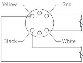
2 Wire Duplex Resistance Thermometer
