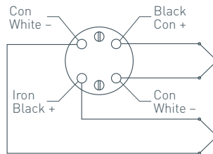
Type J Duplex Thermocouple
