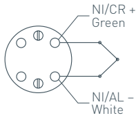
Type K Single Thermocouple
