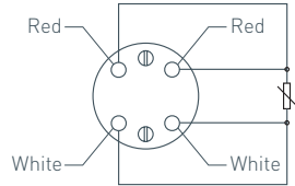
4 Wire Single Resistance Thermometer
