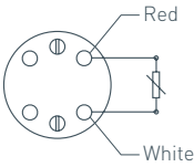
2 Wire Single Resistance Thermometer
