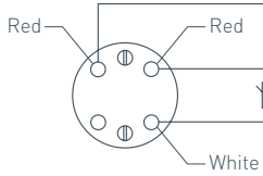
3 Wire Single Resistance Thermometer
